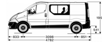
Vivaro DoubleCab L1 H1
