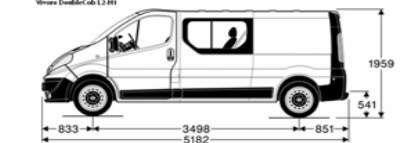
Vivaro DoubleCab L2 H1
